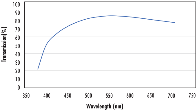
#15-944 Reference Transmission Plot
