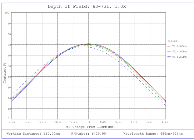
#63-731, 1X, 110mm WD CompactTL™ Telecentric Lens, Depth of Field Plot, 110mm Working Distance, f20.9
