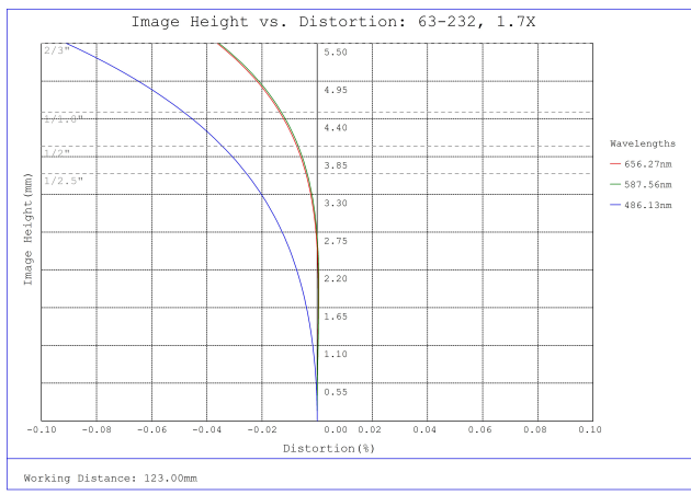
#63-232, 1.7X, 2/3" C-Mount PlatinumTL™ Telecentric Lens, Distortion Plot
