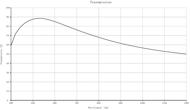
1.7mm FL, f/2.5, Low Distortion M12 Lens, Transmission Plot
