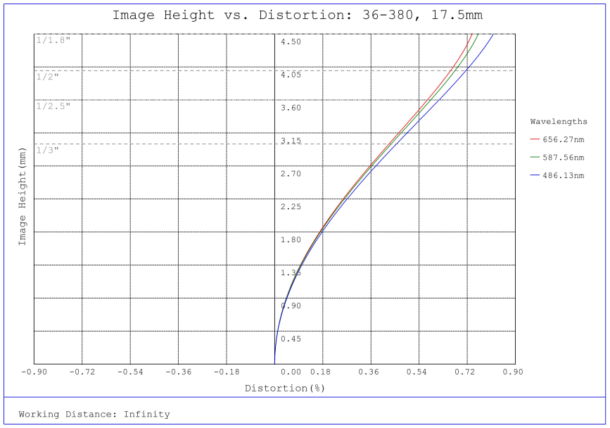
#36-380, 17.5mm FL f/2.5, Rugged Blue Series M12 Lens, Distortion Plot
