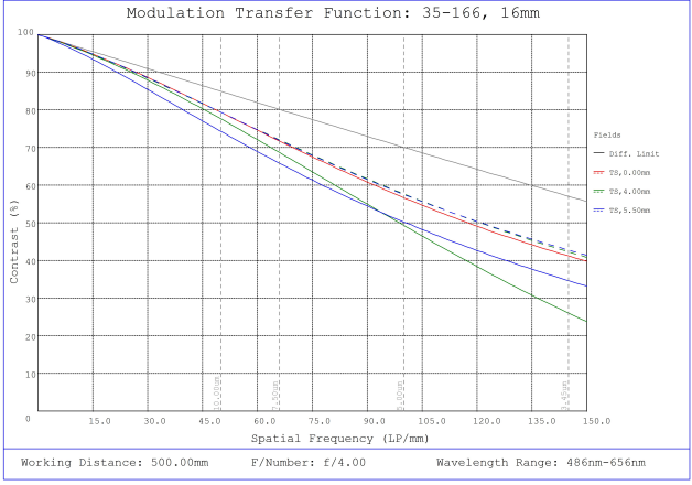
#35-166, 16mm, f/4 Cr Series Fixed Focal Length Lens, Modulated Transfer Function (MTF) Plot, 500mm Working Distance, f4
