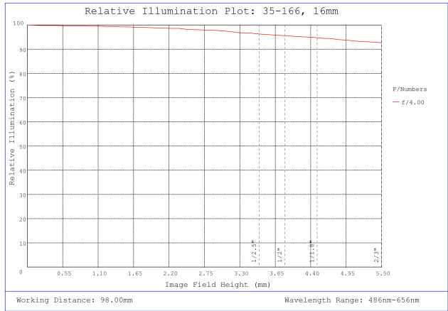
#35-166, 16mm, f/4 Cr Series Fixed Focal Length Lens, Relative Illumination Plot
