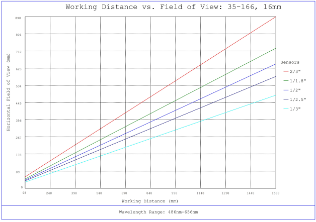
#35-166, 16mm, f/4 Cr Series Fixed Focal Length Lens, Working Distance versus Field of View Plot
