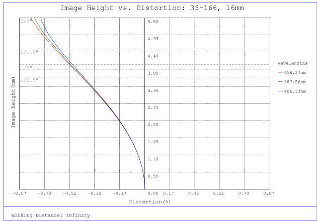
#35-166, 16mm, f/4 Cr Series Fixed Focal Length Lens, Distortion Plot
