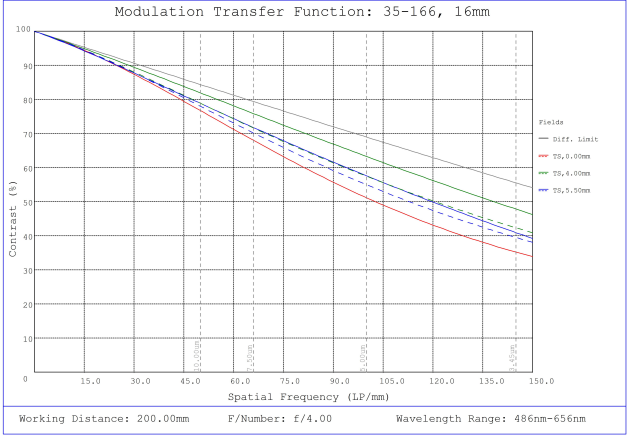
#35-166, 16mm, f/4 Cr Series Fixed Focal Length Lens, Modulated Transfer Function (MTF) Plot, 200mm Working Distance, f4
