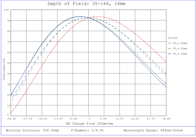
#35-166, 16mm, f/4 Cr Series Fixed Focal Length Lens, Depth of Field Plot, 200mm Working Distance, f4
