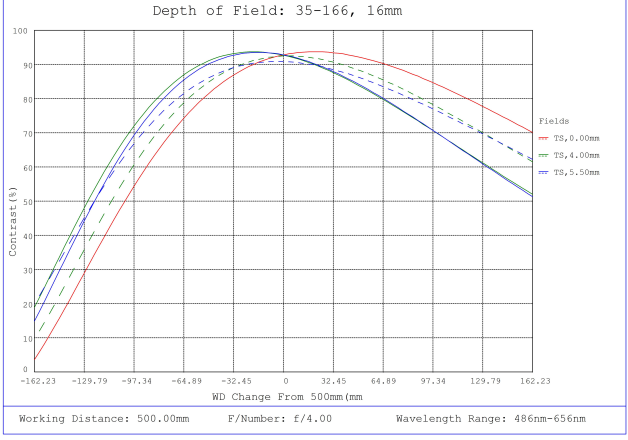
#35-166, 16mm, f/4 Cr Series Fixed Focal Length Lens, Depth of Field Plot, 500mm Working Distance, f4
