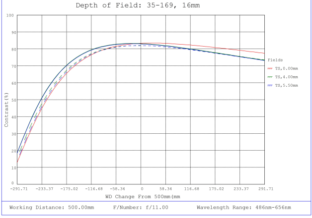
#35-169, 16mm, f/11 Cr Series Fixed Focal Length Lens, Depth of Field Plot, 500mm Working Distance, f11
