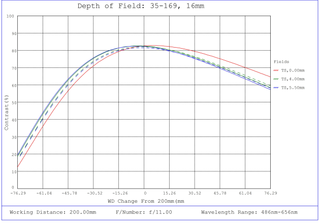
#35-169, 16mm, f/11 Cr Series Fixed Focal Length Lens, Depth of Field Plot, 200mm Working Distance, f11
