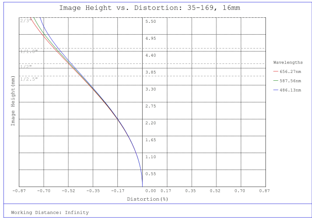
#35-169, 16mm, f/11 Cr Series Fixed Focal Length Lens, Distortion Plot
