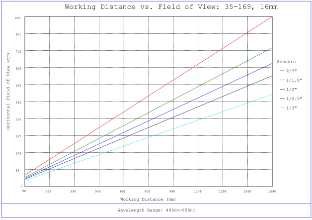
#35-169, 16mm, f/11 Cr Series Fixed Focal Length Lens, Working Distance versus Field of View Plot
