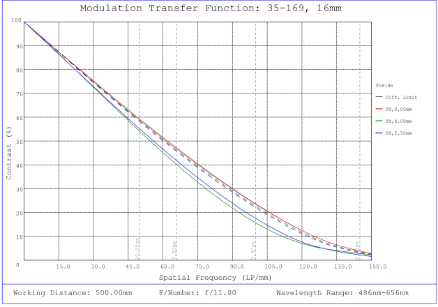
#35-169, 16mm, f/11 Cr Series Fixed Focal Length Lens, Modulated Transfer Function (MTF) Plot, 500mm Working Distance, f11
