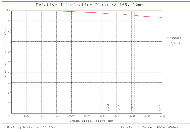
#35-169, 16mm, f/11 Cr Series Fixed Focal Length Lens, Relative Illumination Plot
