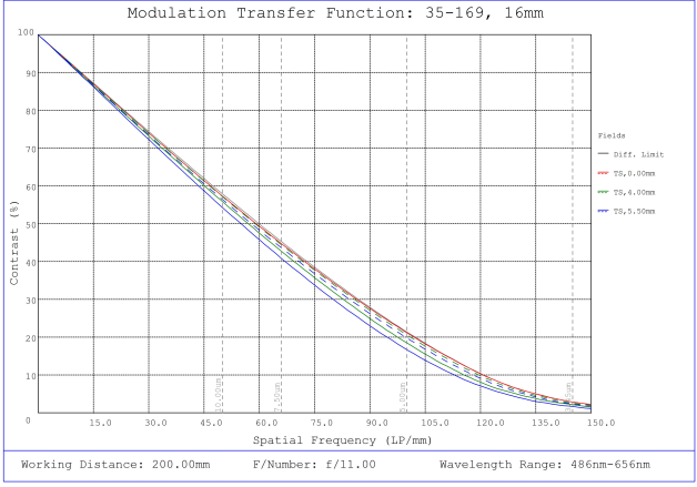
#35-169, 16mm, f/11 Cr Series Fixed Focal Length Lens, Modulated Transfer Function (MTF) Plot, 200mm Working Distance, f11
