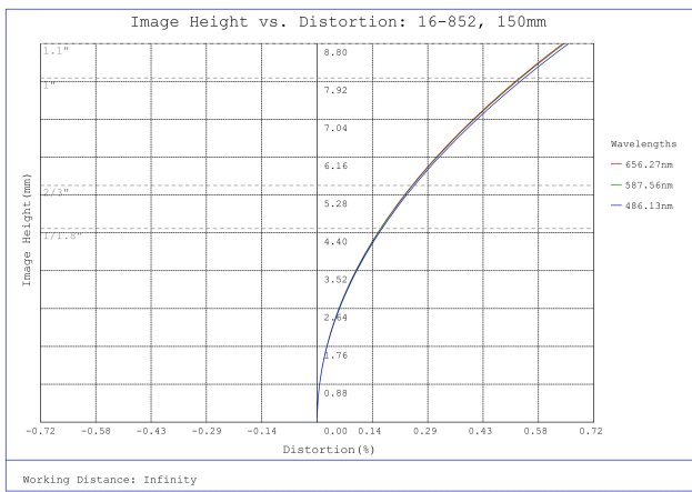
#16-852, 150mm, f/4 Athermal Lens, Distortion Plot
