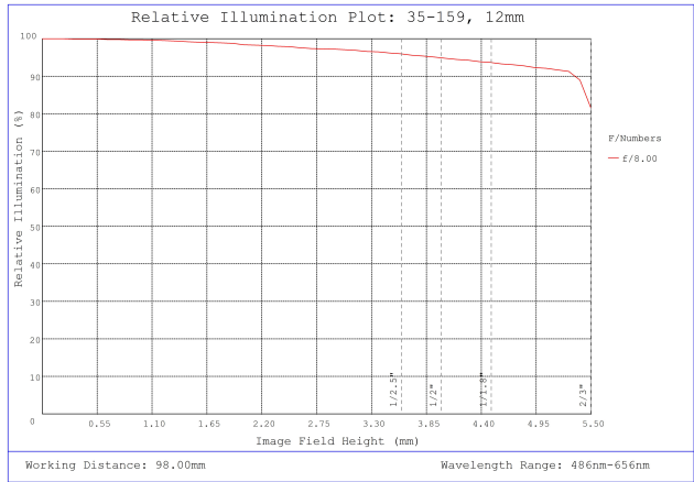
#35-159, 12mm, f/8 Cr Series Fixed Focal Length Lens, Relative Illumination Plot
