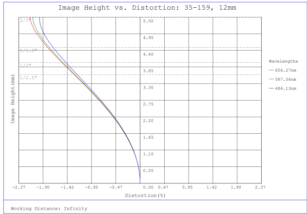
#35-159, 12mm, f/8 Cr Series Fixed Focal Length Lens, Distortion Plot
