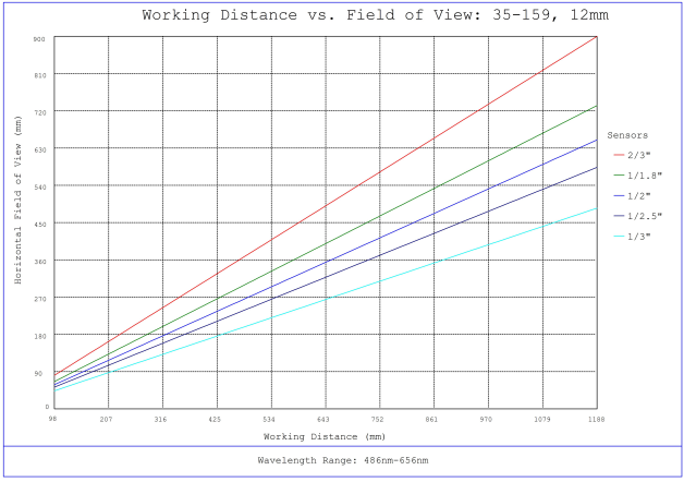
#35-159, 12mm, f/8 Cr Series Fixed Focal Length Lens, Working Distance versus Field of View Plot
