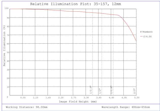
#35-157, 12mm, f/4 Cr Series Fixed Focal Length Lens, Relative Illumination Plot
