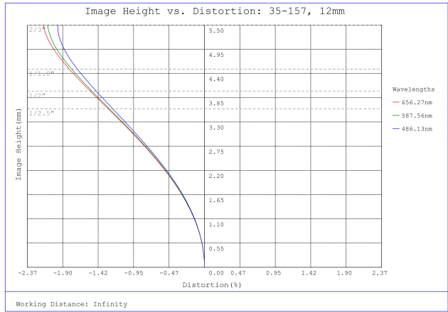
#35-157, 12mm, f/4 Cr Series Fixed Focal Length Lens, Distortion Plot
