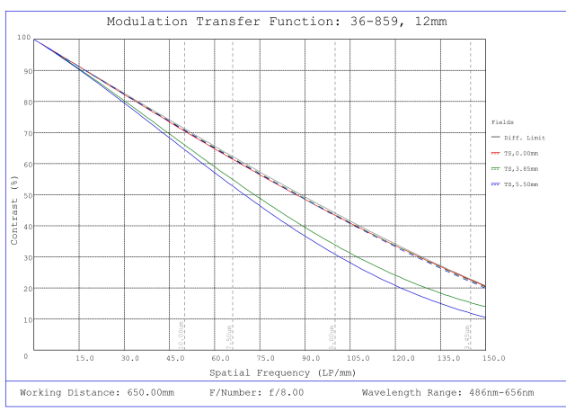
#36-859, 12mm f/8, 400-2000mm Primary WD, HRr Series Fixed Focal Length Lens, Modulated Transfer Function (MTF) Plot, 650mm Working Distance, f8
