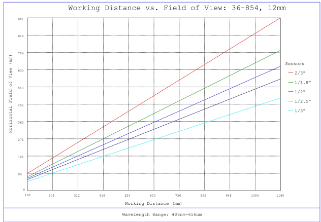
#36-854, 12mm f/4, 1000mm-∞ Primary WD, HRr Series Fixed Focal Length Lens, Working Distance versus Field of View Plot
