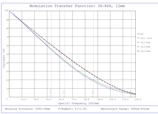
#36-864, 12mm f/11, 1000mm-∞ Primary WD, HRr Series Fixed Focal Length Lens, Modulated Transfer Function (MTF) Plot, 1000mm Working Distance, f11
