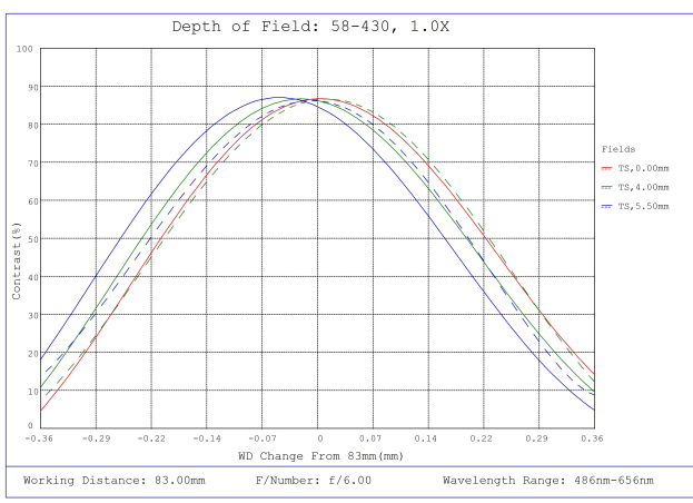
#58-430, 1.0X SilverTL™ Telecentric Lens, Depth of Field Plot, 83mm Working Distance, f6
