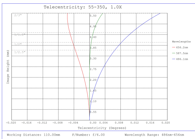
#55-350, 1.0X 2/3" GoldTL™ Telecentric Lens, Telecentricity Plot
