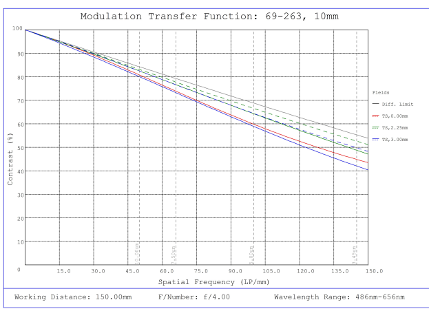
#69-263, 10mm FL f/4, Blue Series M12 Lens, Modulated Transfer Function (MTF) Plot, 150mm Working Distance, f4
