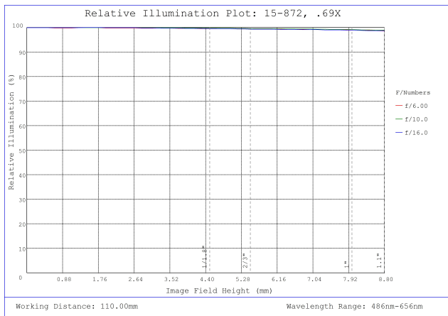
#15-872, 0.69X CobaltTL Telecentric Lens, Relative Illumination Plot
