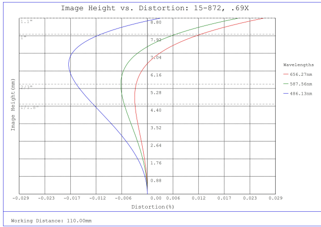
#15-872, 0.69X CobaltTL Telecentric Lens, Distortion Plot
