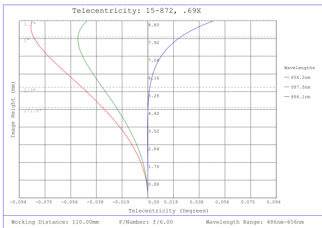
#15-872, 0.69X CobaltTL Telecentric Lens, Telecentricity Plot
