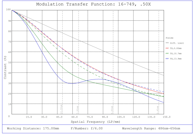
#16-749, 0.5X, 28.7mm TFL-Mount PlatinumTL™ Telecentric Lens, Modulated Transfer Function (MTF) Plot, 175mm Working Distance, f6
