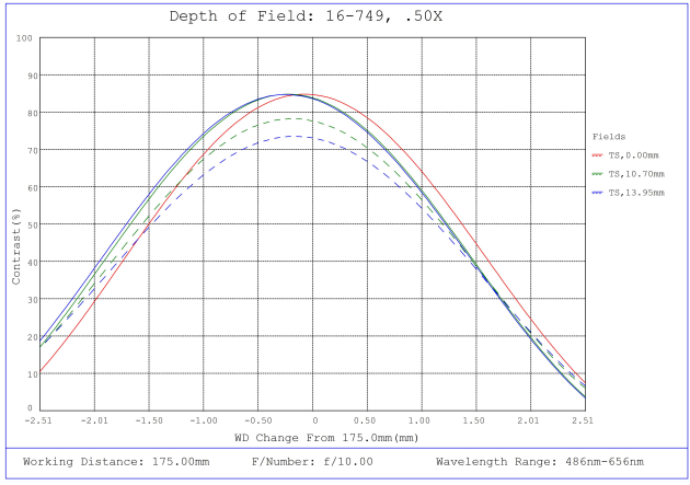
#16-749, 0.5X, 28.7mm TFL-Mount PlatinumTL™ Telecentric Lens, Depth of Field Plot, 175mm Working Distance, f10
