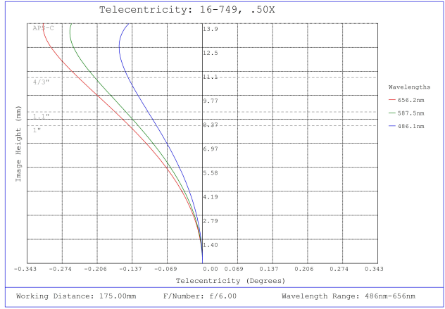
#16-749, 0.5X, 28.7mm TFL-Mount PlatinumTL™ Telecentric Lens, Telecentricity Plot
