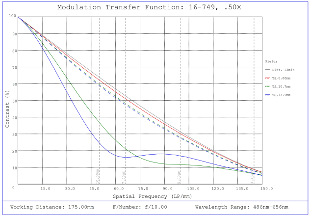
#16-749, 0.5X, 28.7mm TFL-Mount PlatinumTL™ Telecentric Lens, Modulated Transfer Function (MTF) Plot, 175mm Working Distance, f10
