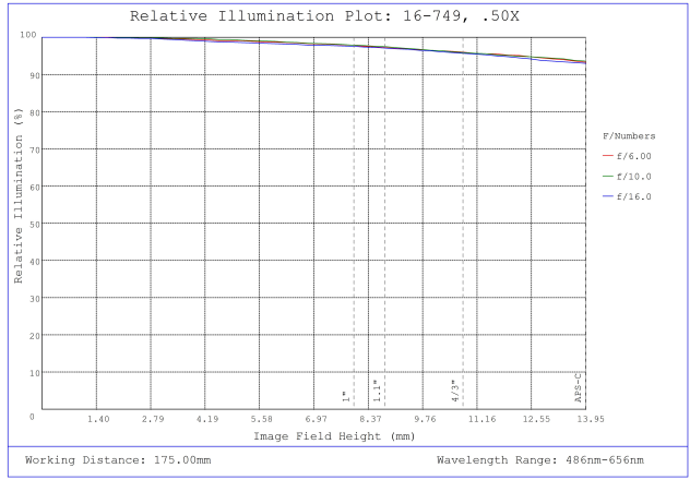
#16-749, 0.5X, 28.7mm TFL-Mount PlatinumTL™ Telecentric Lens, Relative Illumination Plot
