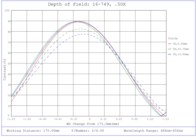
#16-749, 0.5X, 28.7mm TFL-Mount PlatinumTL™ Telecentric Lens, Depth of Field Plot, 175mm Working Distance, f6
