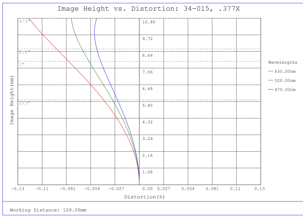
#34-015, 0.377X, 4/3" C-Mount TitanTL® Telecentric Lens, Distortion Plot
