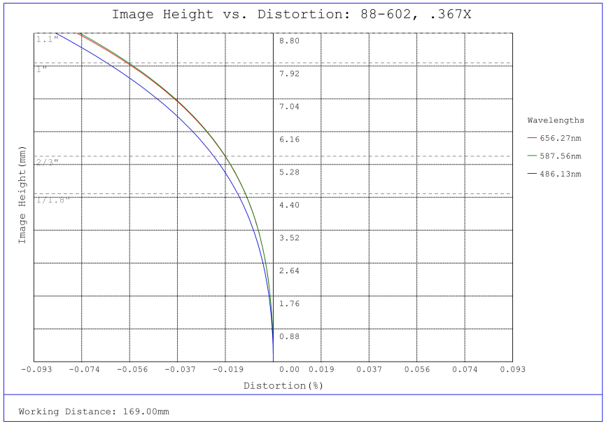
#88-602, 0.367X CobaltTL Telecentric Lens, Distortion Plot
