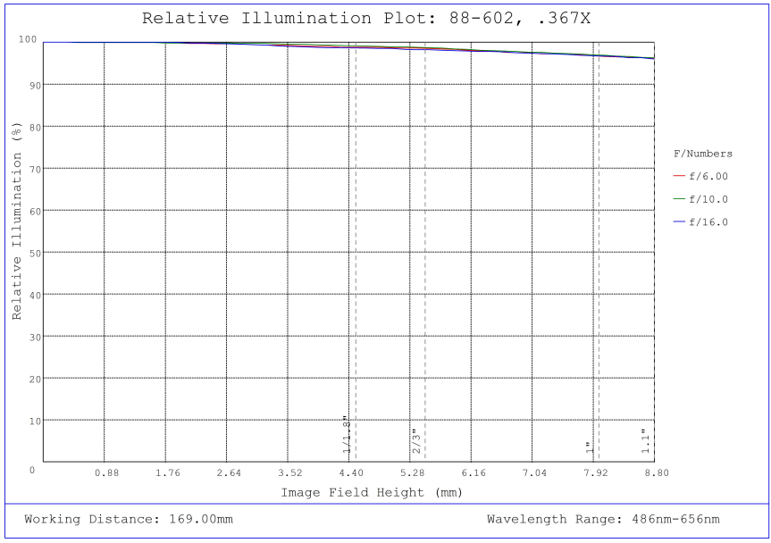
#88-602, 0.367X CobaltTL Telecentric Lens, Relative Illumination Plot
