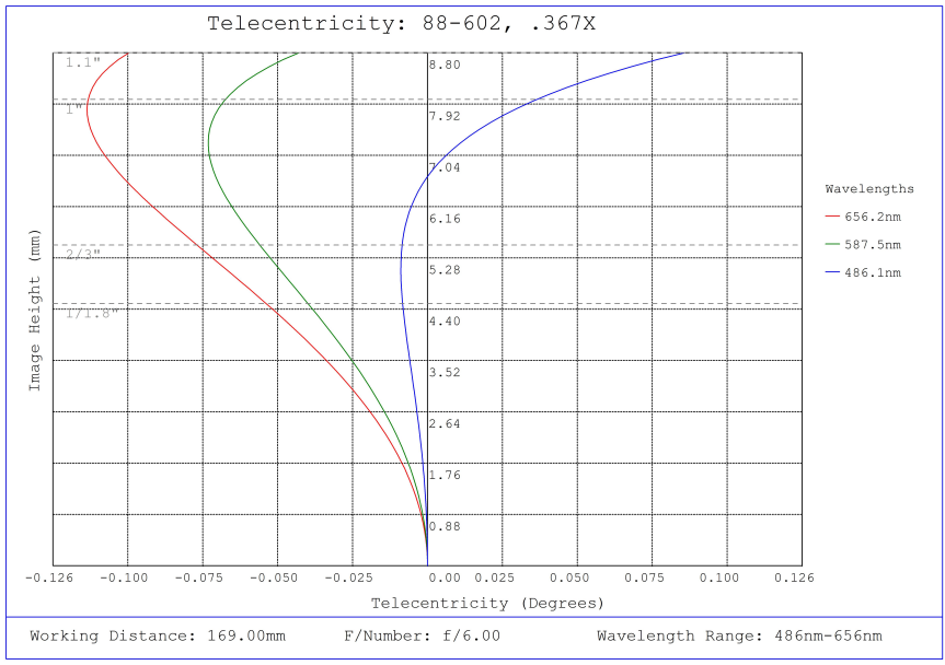
#88-602, 0.367X CobaltTL Telecentric Lens, Telecentricity Plot
