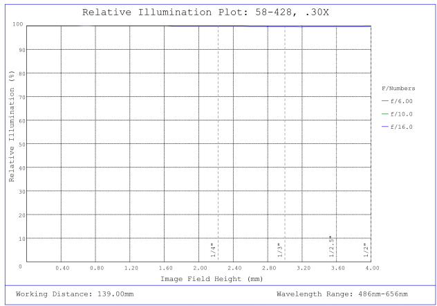
#58-428, 0.30X SilverTL™ Telecentric Lens, Relative Illumination Plot
