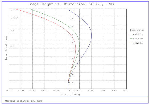
#58-428, 0.30X SilverTL™ Telecentric Lens, Distortion Plot
