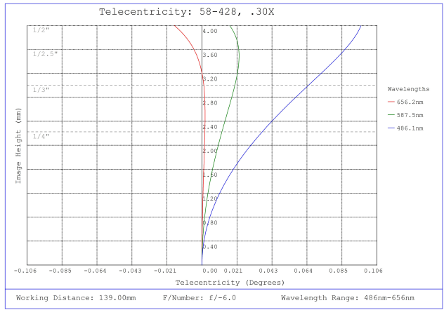
#58-428, 0.30X SilverTL™ Telecentric Lens, Telecentricity Plot
