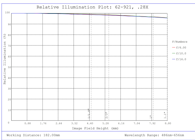
#62-921, 0.28X CobaltTL Telecentric Lens, Relative Illumination Plot
