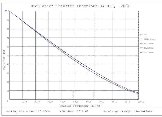
#34-010, 0.268X, 1" C-Mount TitanTL® Telecentric Lens, Modulated Transfer Function (MTF) Plot, 110mm Working Distance, f16
