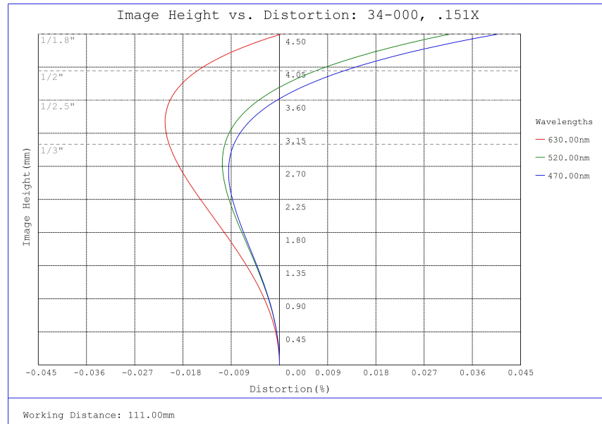
#34-000, 0.151X, 1/1.8" C-Mount TitanTL® Telecentric Lens, Distortion Plot
