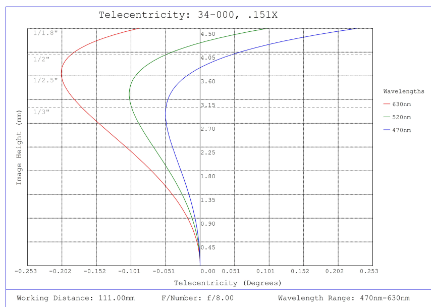
#34-000, 0.151X, 1/1.8" C-Mount TitanTL® Telecentric Lens, Telecentricity Plot
