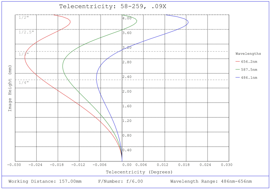
#58-259, 0.09X ½" GoldTL™ Telecentric Lens, Telecentricity Plot
