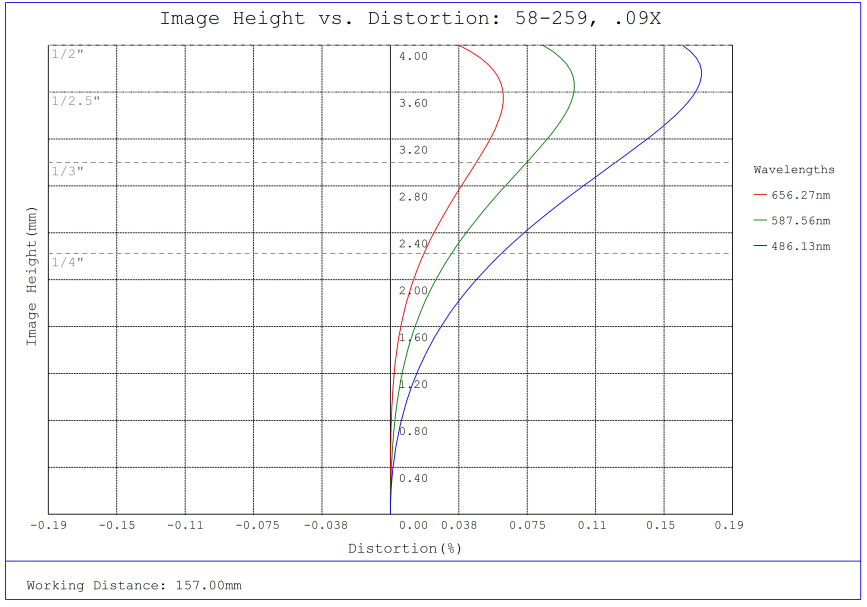
#58-259, 0.09X ½" GoldTL™ Telecentric Lens, Distortion Plot
