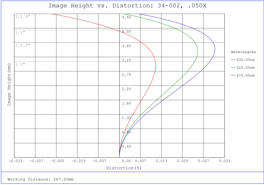
#34-002, 0.050X, 1/1.8" C-Mount TitanTL® Telecentric Lens, Distortion Plot
