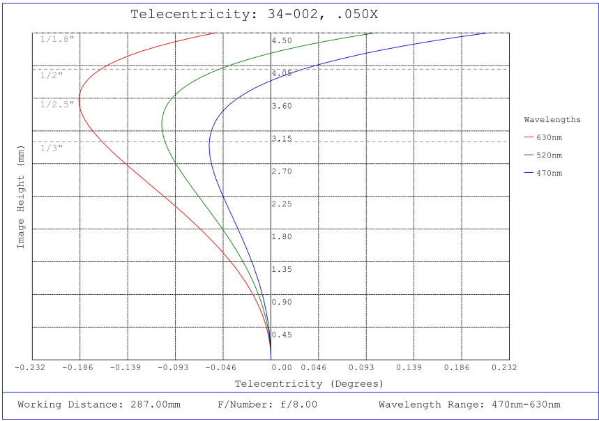
#34-002, 0.050X, 1/1.8" C-Mount TitanTL® Telecentric Lens, Telecentricity Plot
