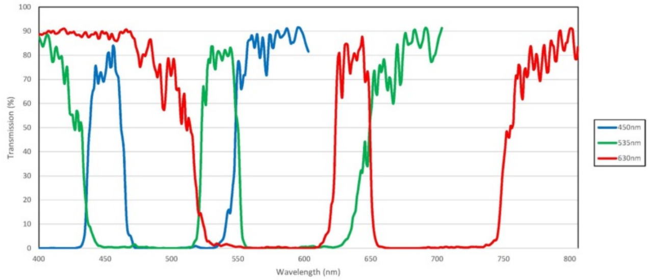
Everix Ultra-Thin Broadband Bandpass Filter Coating Curve
