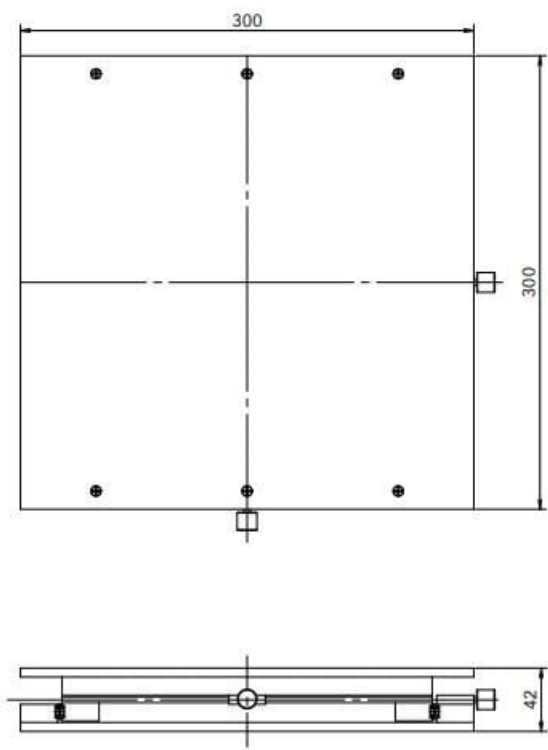
#55-620, 200mm Travel, X-Y Positioning Table (Units: mm)
