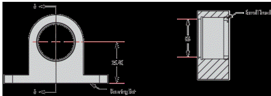
Side Flange Type (#36-414 & #36-418)
