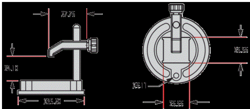
Cube Beamsplitter Type (#36-415)
