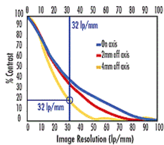
Modulation Transfer Function—1X PMAG Object Resolution (lp/mm)
