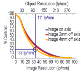
Modulation Transfer Function @ 3.0X PMAG
