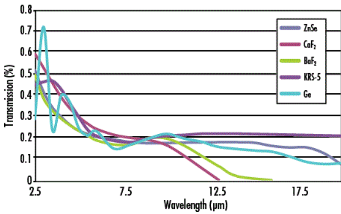
Typical Min Transmission for Linear Polarized Light
