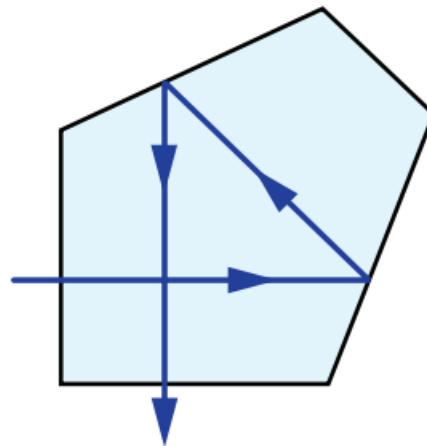
Penta Prism Ray Path
