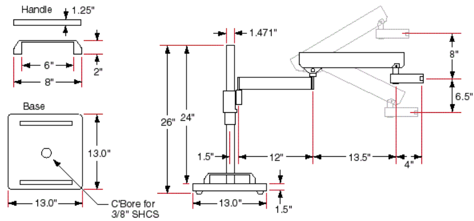
#54-119 Articulating Arm Boom Stand
