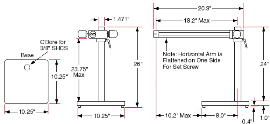
#54-120 Standard Boom Stand
